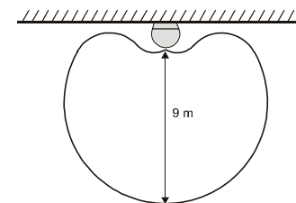
glass break detector working range diagram
